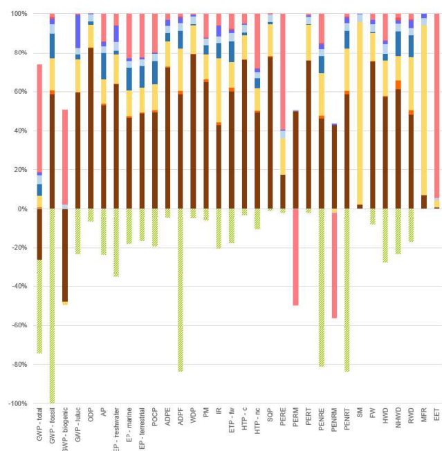
Figure : Indicator results of direct pressure laminate floor covering over its life cycle
